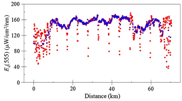
Fig. 3. An example of E_d(h, 555, t) before and after wavelet transform; red: discarded data; blue: valid data after wavelet transform.
