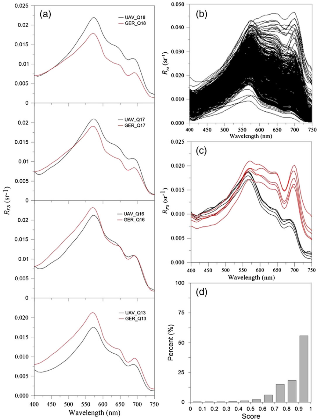
Fig. 6. (a) R_{rs-u} compared to concurrent R_{rs-f} measured in Weitou Bay (4 match-ups available); (b) all R_{rs-u} collected over Weitou Bay ( n = 697 ); (c) examples of R_{rs-u} showing strong peaks around 700 nm (red curves) compared to R_{rs-u} with peaks around 683 nm (black curves); (d) frequency distribution of scores of all R_{rs-u} evaluated by a quality assurance system (Wei et al., 2016).
